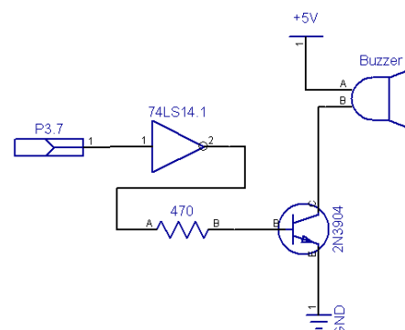
Gambar 6 Rangkaian Buzzer
