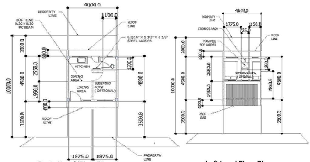
Basic Unit G/Floor Plan
