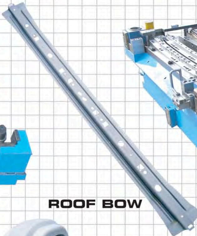
PROGRESSIVE DIE 12 STATION, ONE OUT (LOWER)
