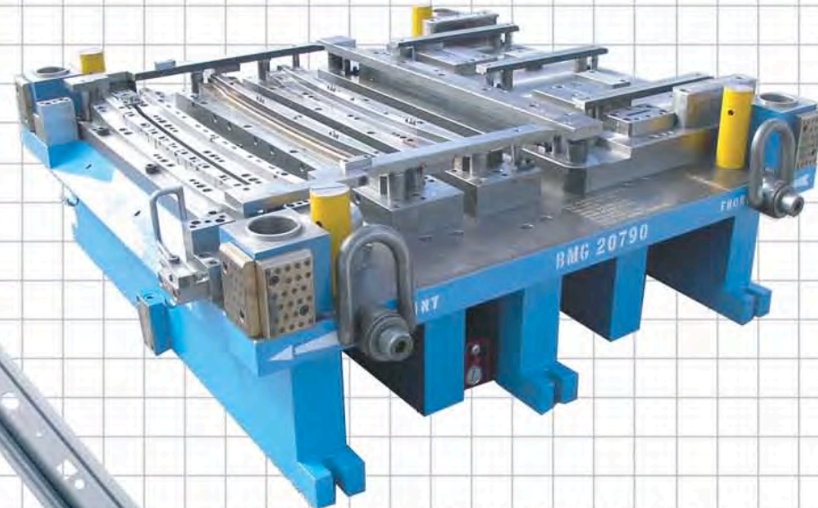
PROGRESSIVE DIE 12 STATION, ONE OUT (LOWER)
