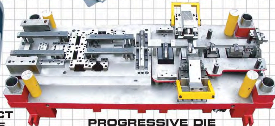
PROGRESSIVE DIE 12 STATION, ONE OUT (LOWER)
