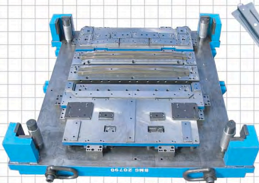
PROGRESSIVE DIE 12 STATION, ONE OUT (UPPER)
