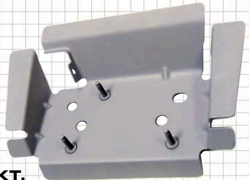
SUPPORT BRKT. HEAVY BLANKING (3/4") MACHINING, FORMING
