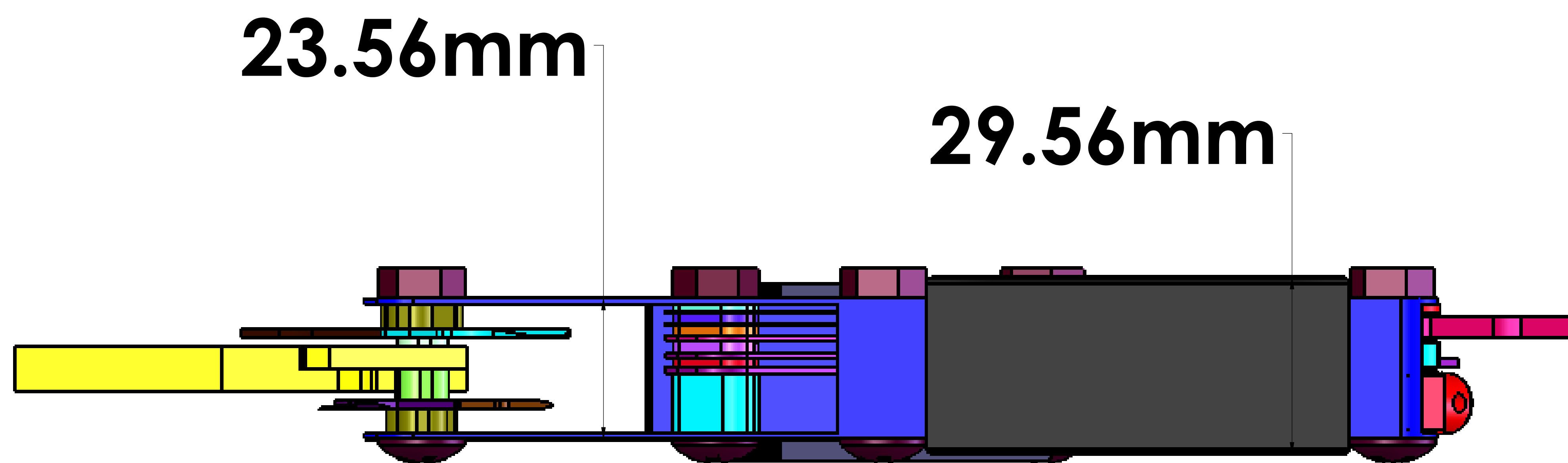
TOP VIEW
