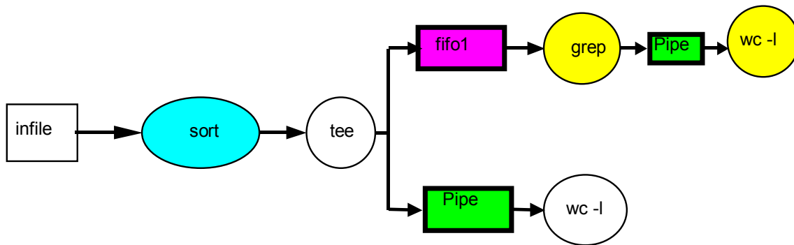
Figure 10.4 Pictorial representation of the semantics of the above shell session
