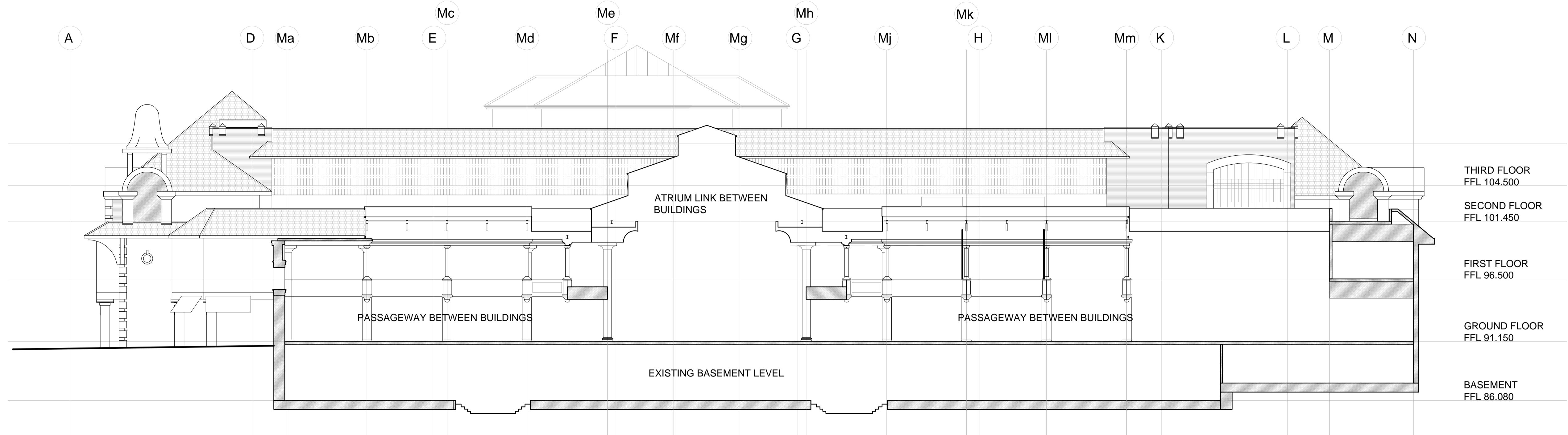
1 EXISTING SECTION C-C SCALE 1:200
