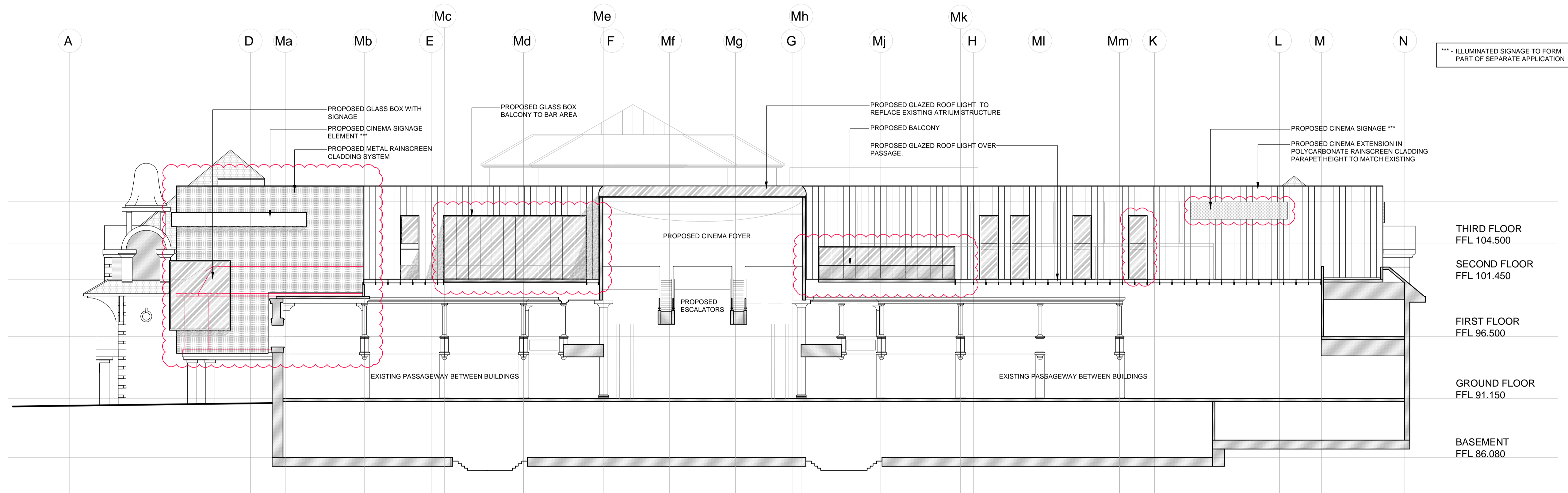
2 PROPOSED SECTION C-C SCALE 1:200
