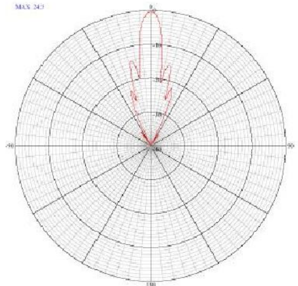
Co-Pol - 0 deg Cut
