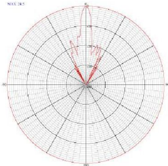
Co-Pol - 90 deg Cut
