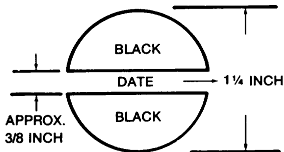
Figure 1-1. MIL-C-46168 Identifier Symbol
