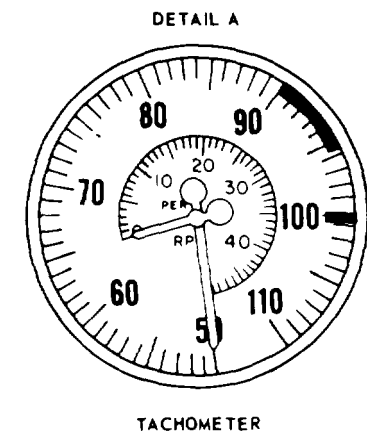
TACHOMETER
