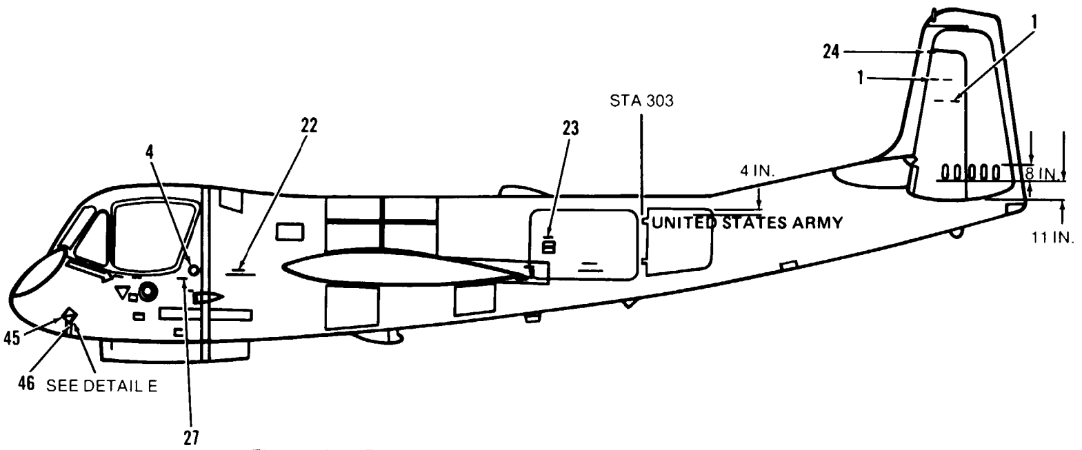
Figure 10-4. Exterior Markings, OV-1D and RV-1D (Sheet 1 of 15).
