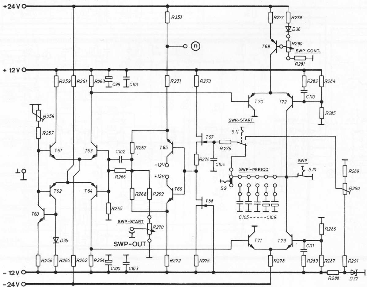
Sweep-Generator
