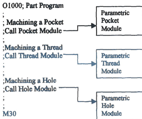
Fig. 1 Feature-Based CNC Program Using Parametric Modules
