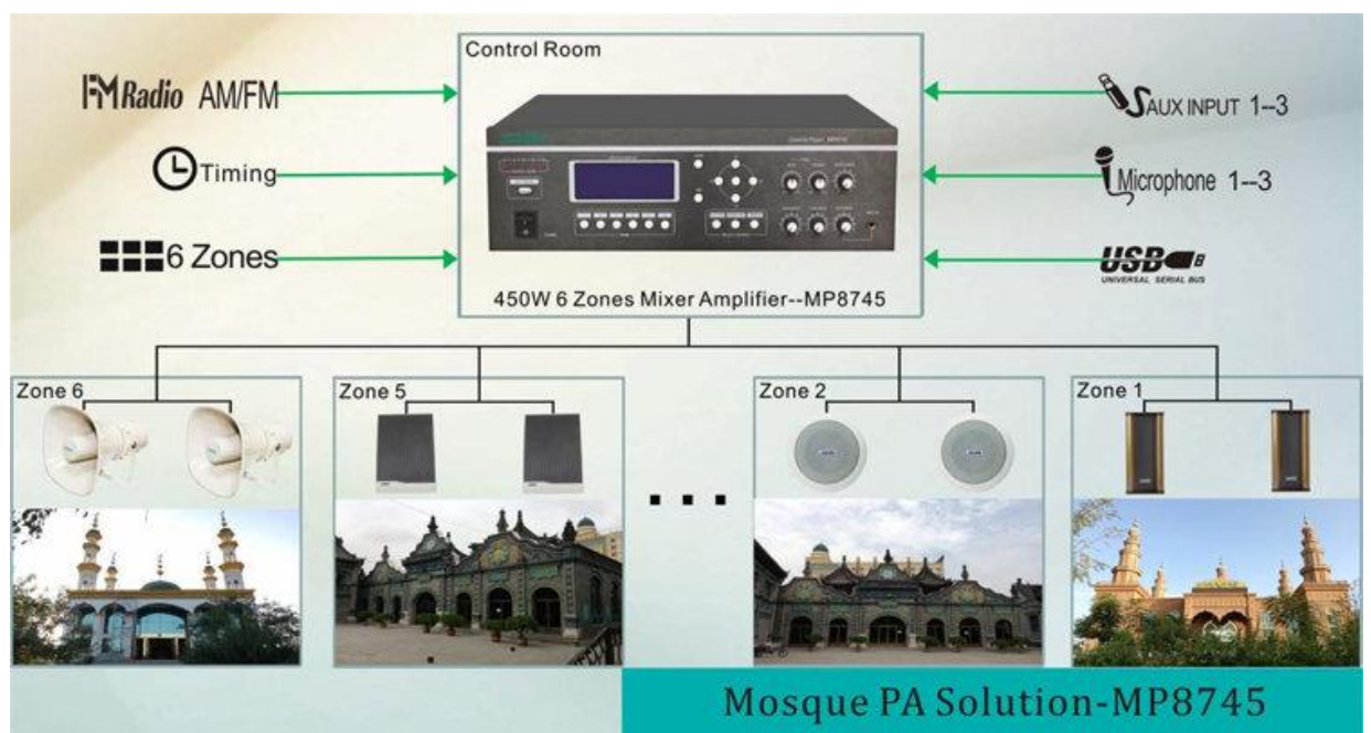
6 Zones PA system,PA Speaker distribution
