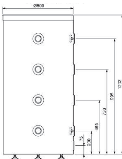
VPS R 200 (200л)
