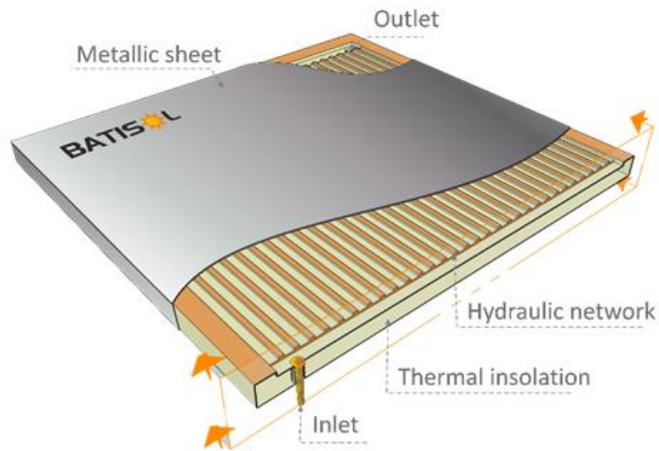
Fig. 3 Conceptual design of the BATISOL collector
