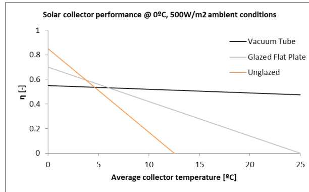
Fig. 1 Efficiency of solar collectors depending on collector temperature for given ambient conditions.
