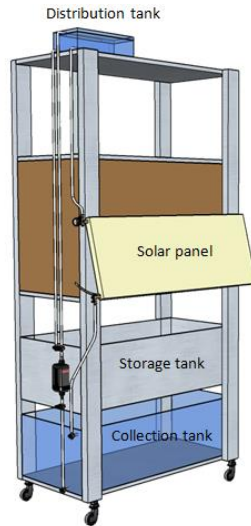
Fig. 6 Schematic of the test bench
