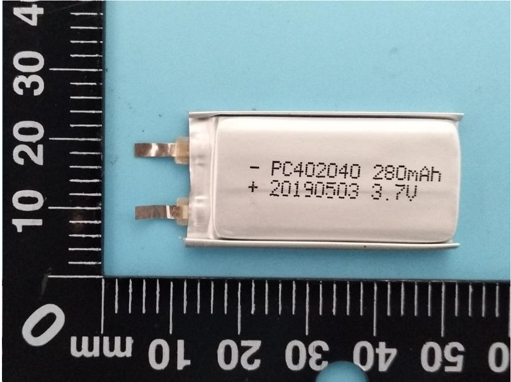
Cell /电芯 (PC402040 3.7V 280mAh 1.036Wh)
