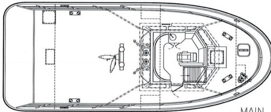
MAIN DECK
