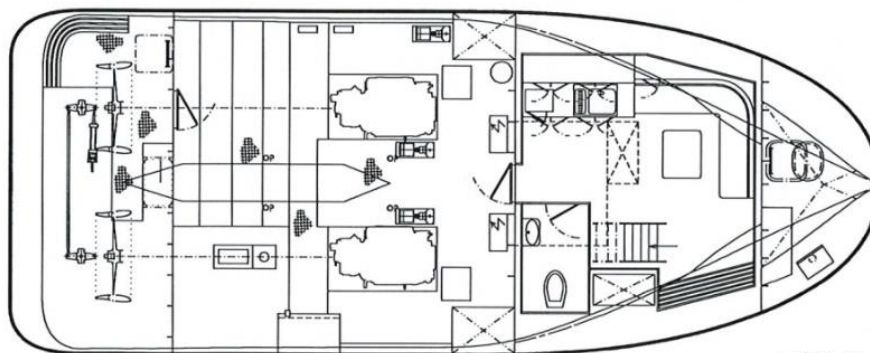
HOLD PLAN
